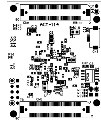
Solder Side
