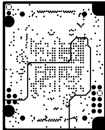
INTERNAL PLANE2
