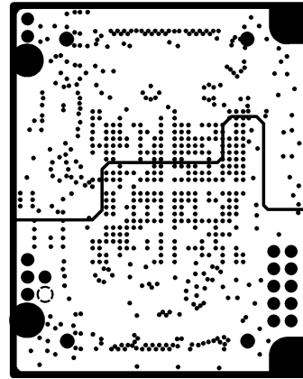
INTERNAL PLANE3
