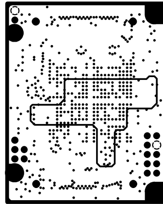
INTERNAL PLANE4
