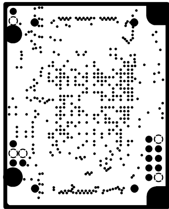
INTERNAL PLANE1
