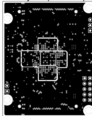
Mid-Layer 2 (Scale 1:1)
