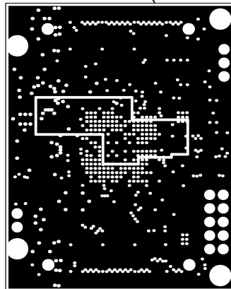
Internal Plane 3 (Scale 1:1)
