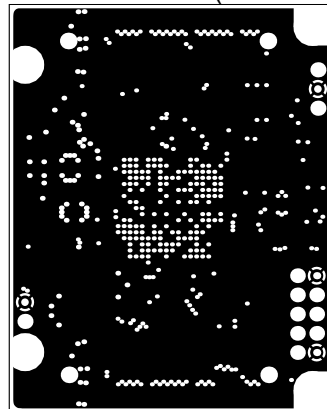
Internal Plane 1 (Scale 1:1)
