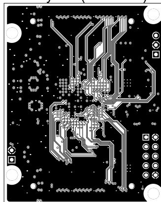
Mid-Layer 1 (Scale 1:1)
