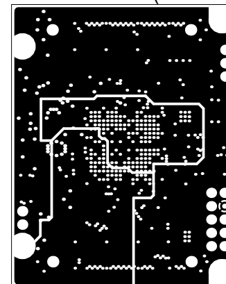
Internal Plane 2 (Scale 1:1)
