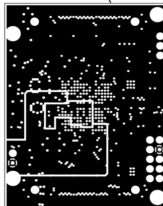
Internal Plane 4 (Scale 1:1)
