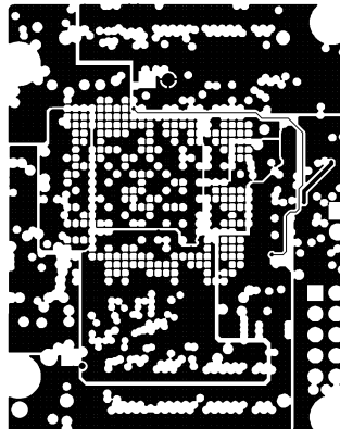
MID LAYER4
