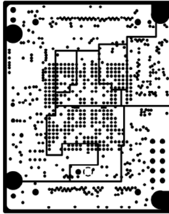
INTERNAL PLANE3
