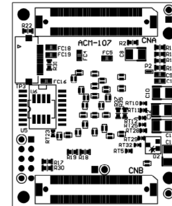
Solder Side
