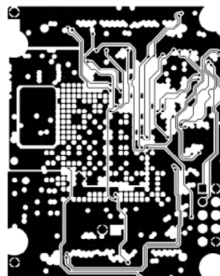
INTERNAL PLANE3
