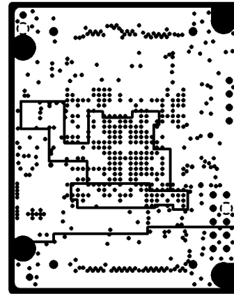
INTERNAL PLANE3
