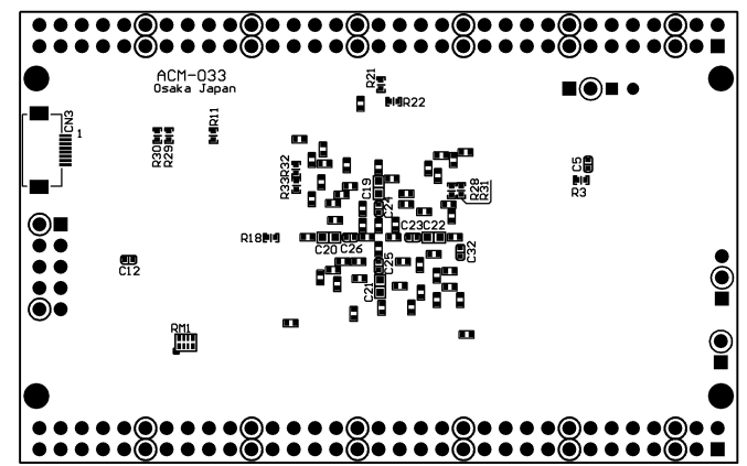
Solder Side
