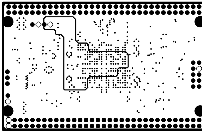
INTERNAL PLANE2
