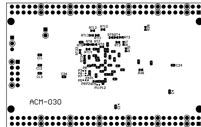
Solder Side
