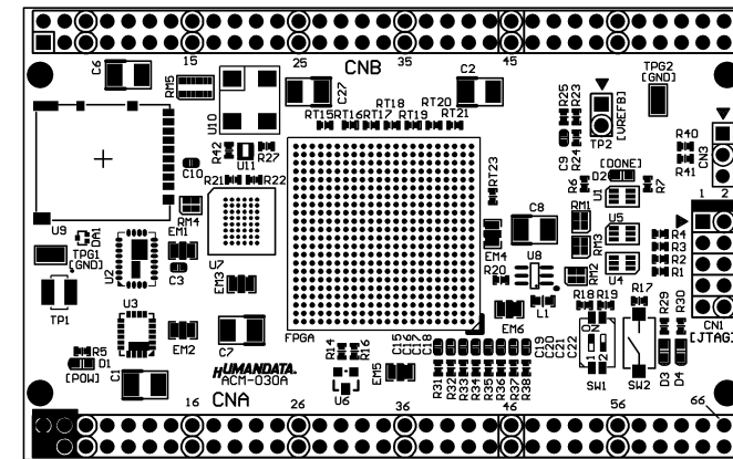
Component Side
