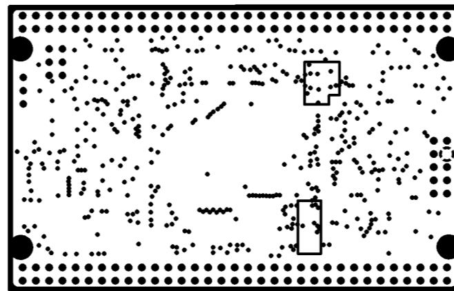
INTERNAL PLANE2
