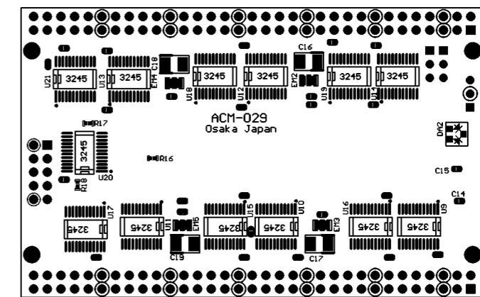
Solder Side
