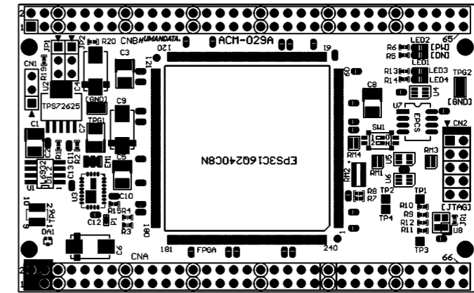
Component Side
