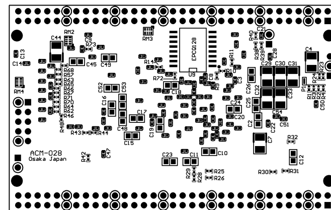
Solder Side
