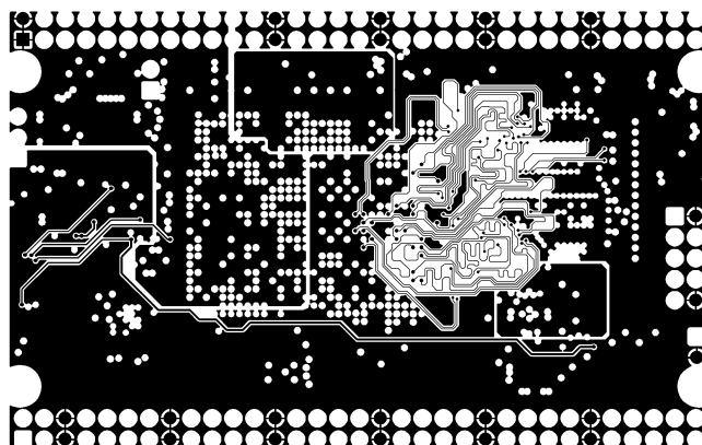
MID LAYER4
