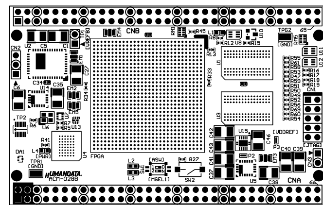
Component Side
