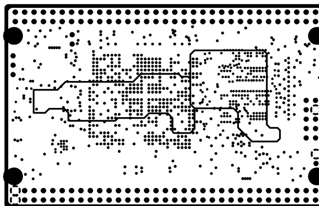
INTERNAL PLANE2
