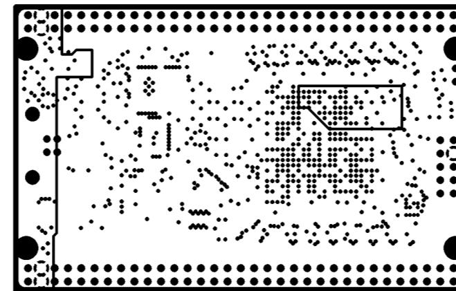
INTERNAL PLANE(VCC)
