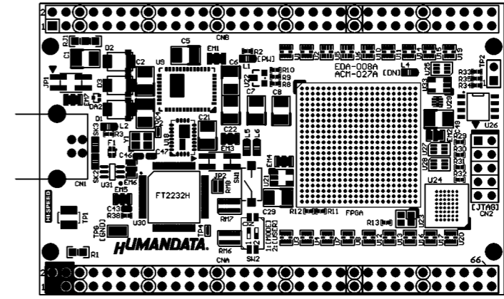
Component Side
