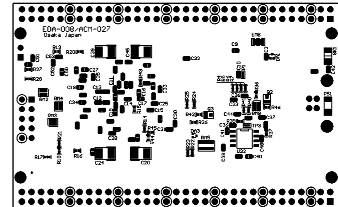
Solder Side
