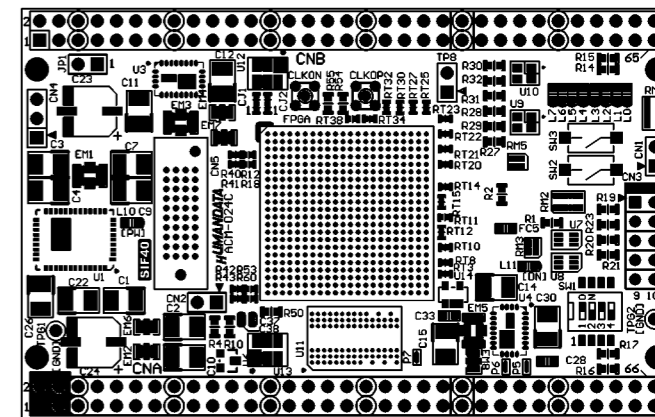
Component Side
