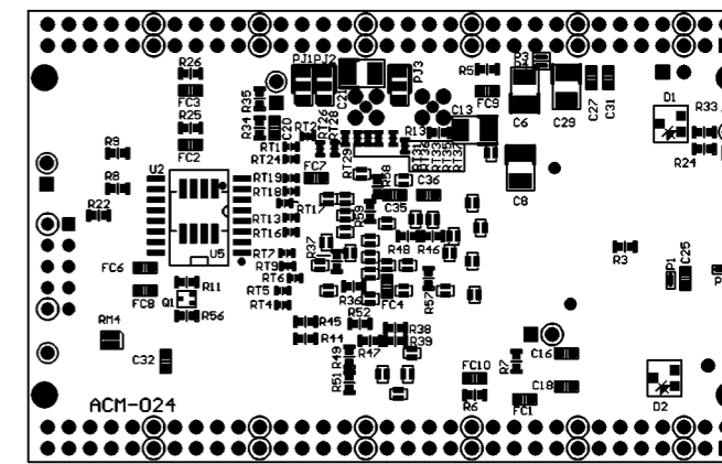
Solder Side
