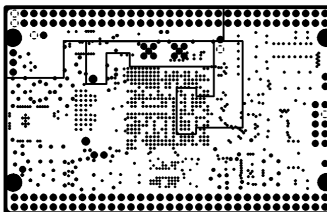
INTERNAL PLANE2
