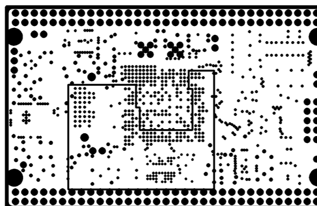
INTERNAL PLANE3
