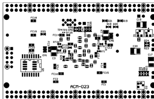
Solder Side
