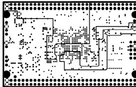
INTERNAL PLANE(VCC)
