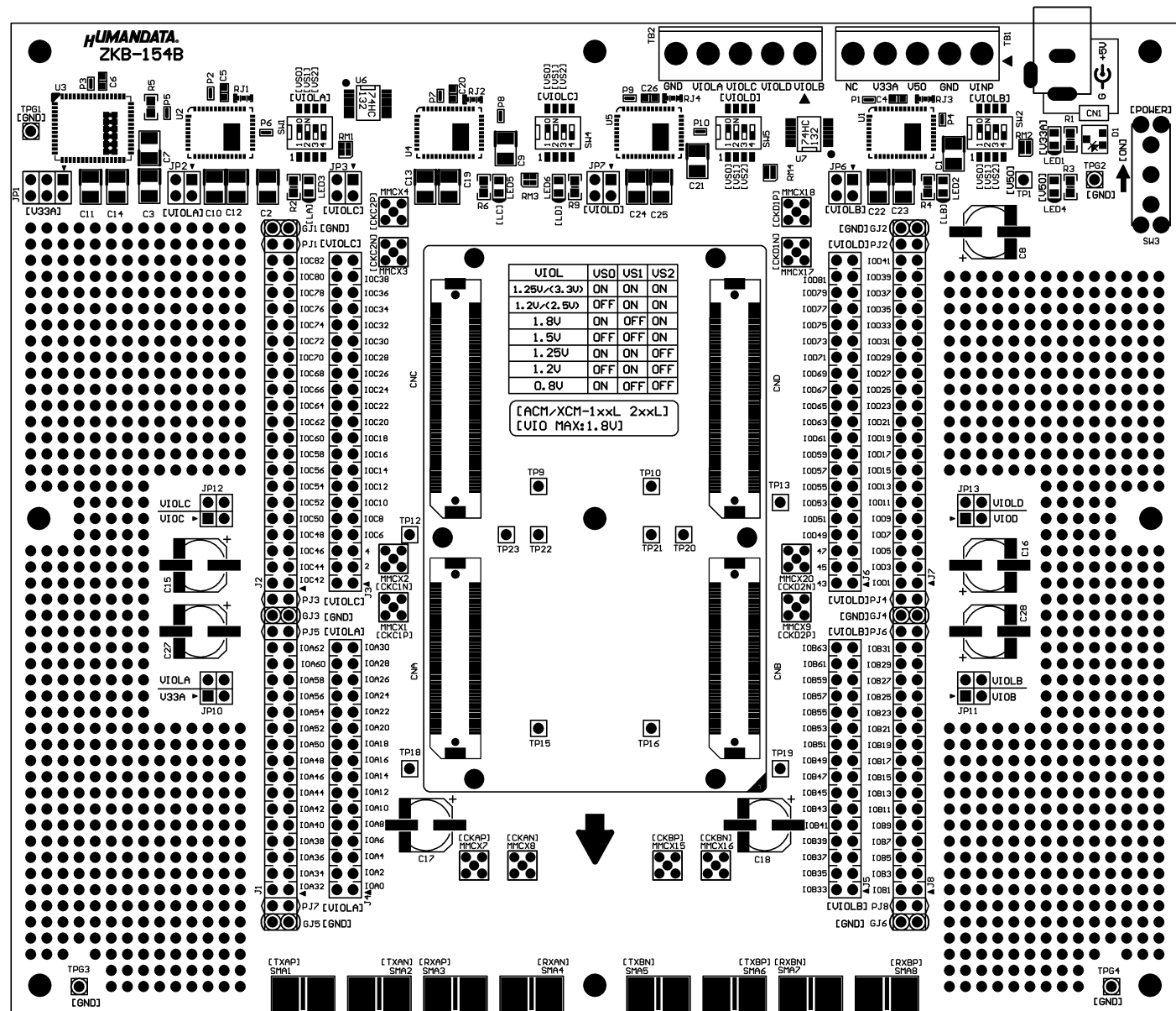
Component Side
