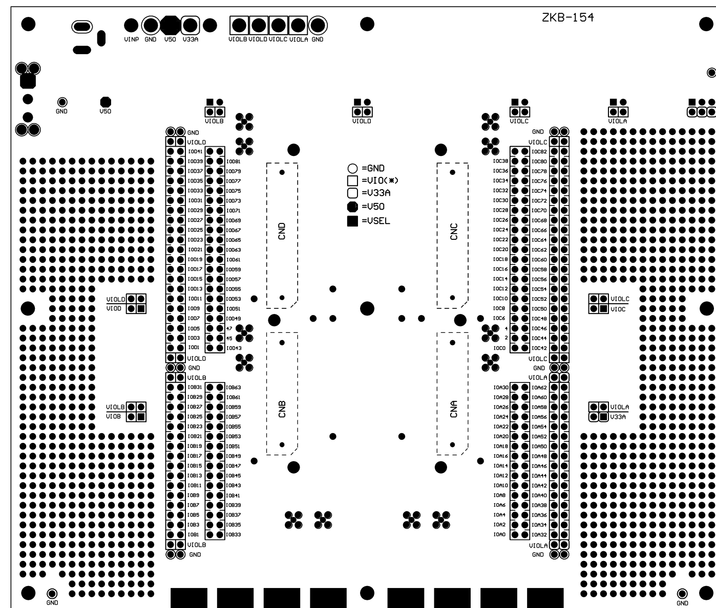
Solder Side
