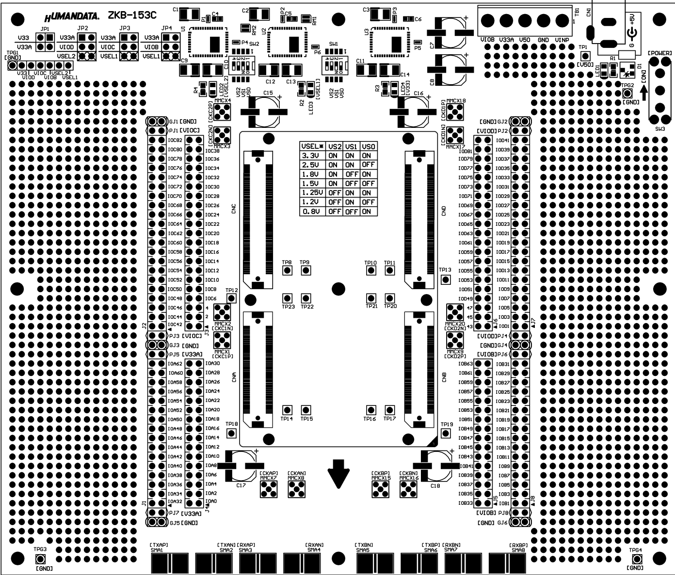
Component Side
