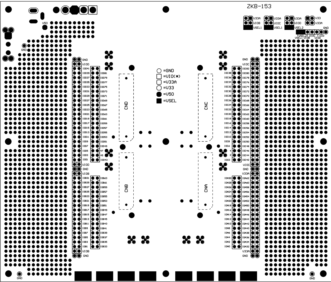
Solder Side
