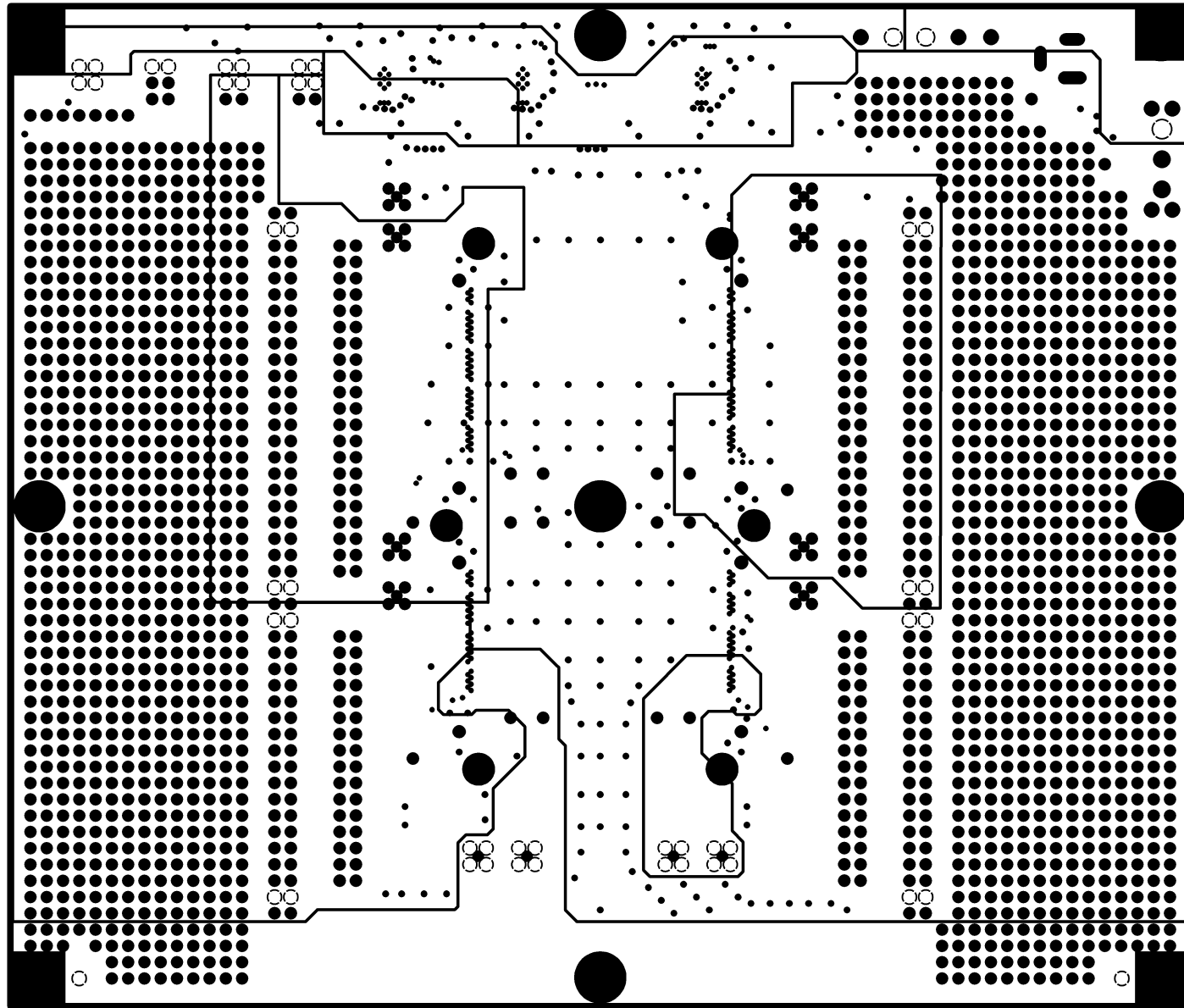
INTERNAL PLANE2
