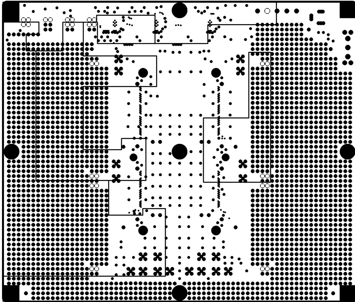
INTERNAL PLANE2
