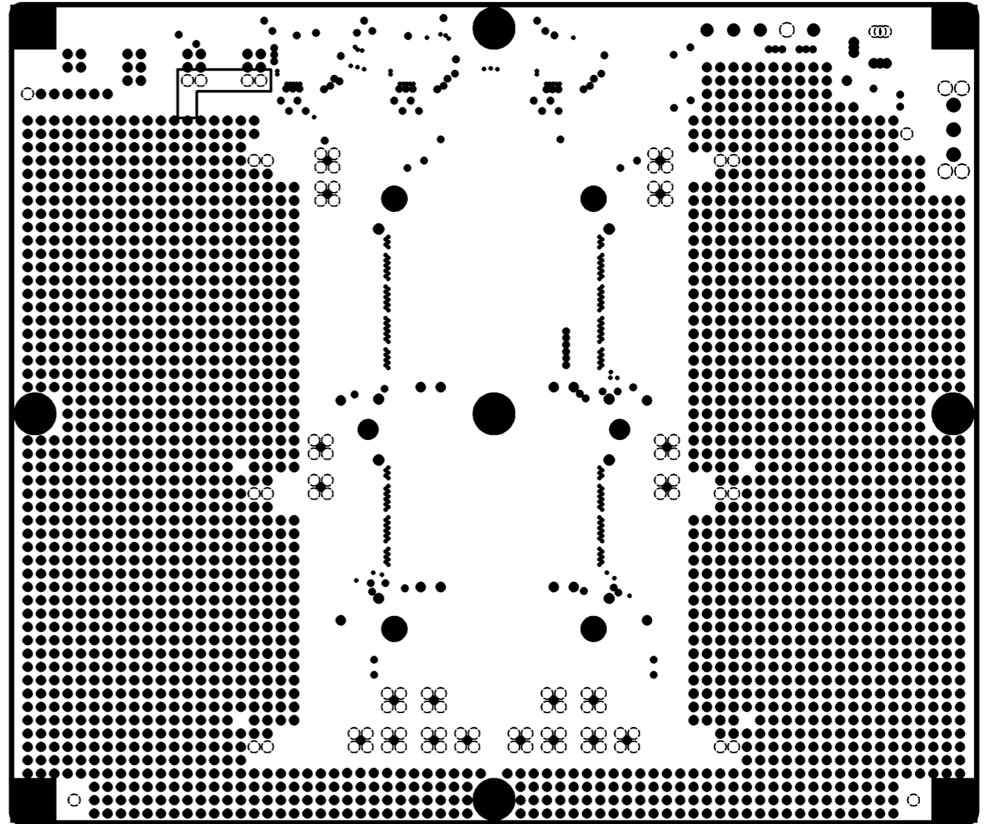
INTERNAL PLANE1
