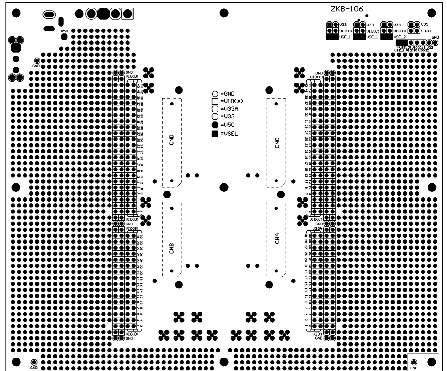
Solder Side
