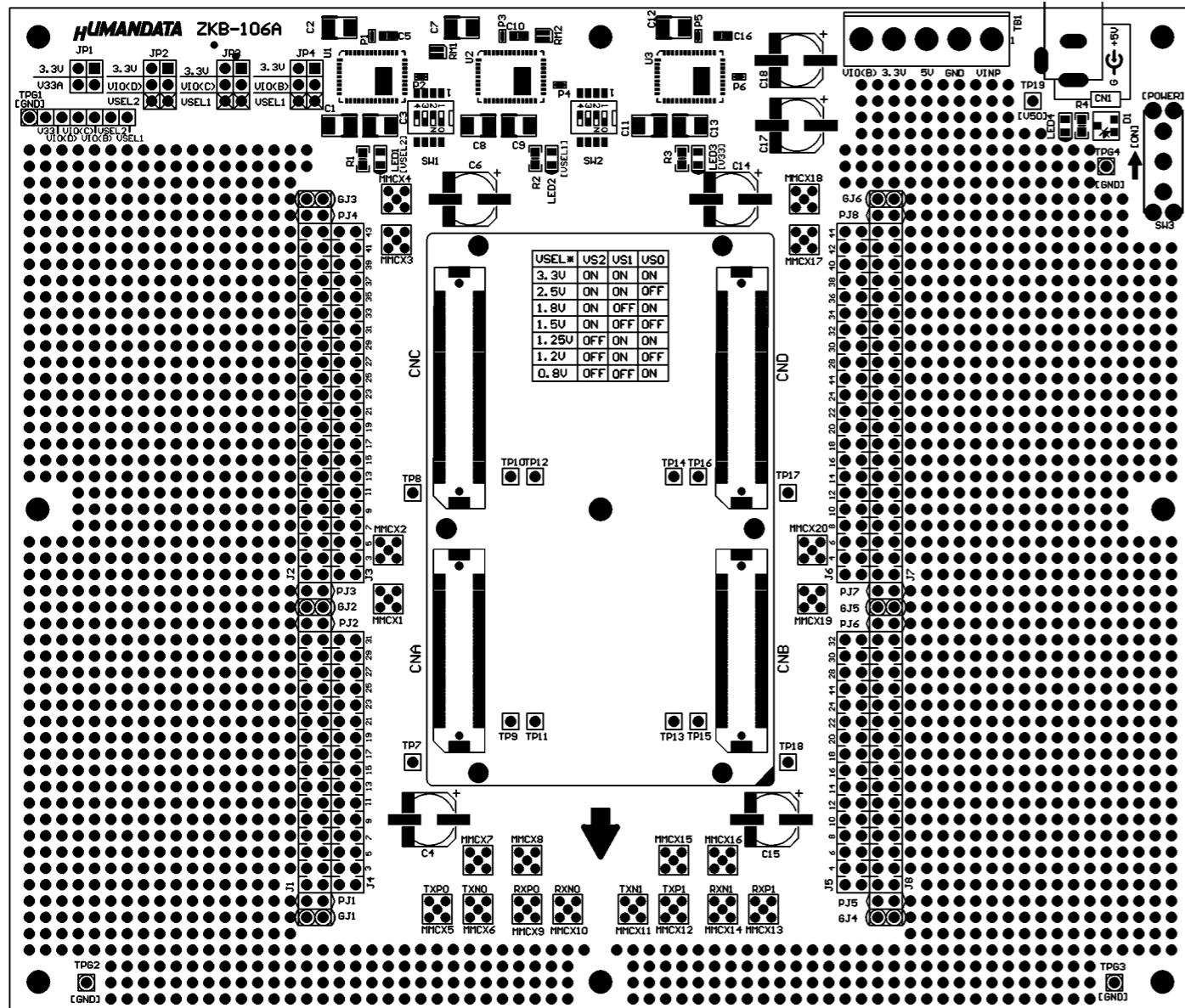
Component Side
