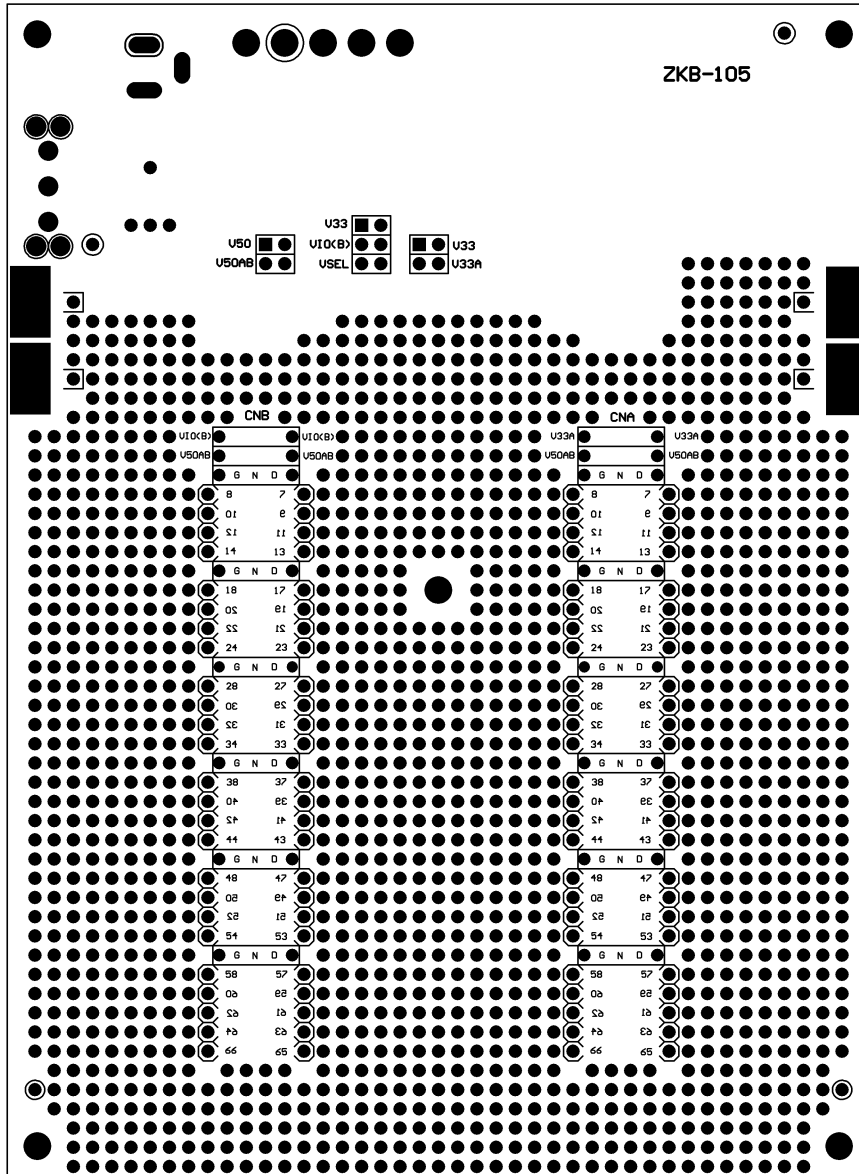
Solder Side
