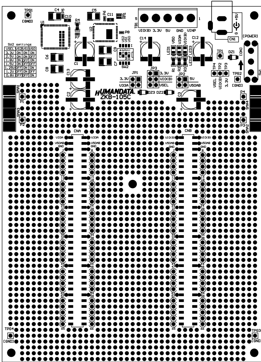
Component Side
