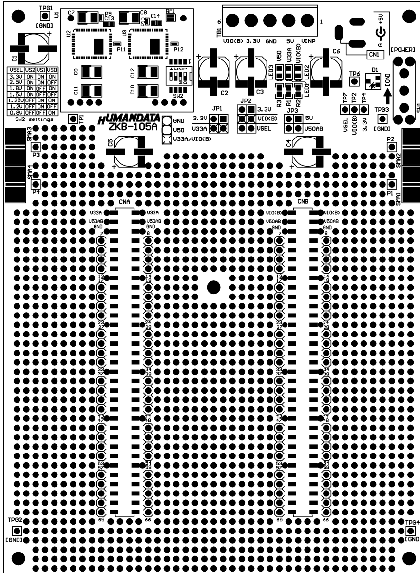
Component Side
