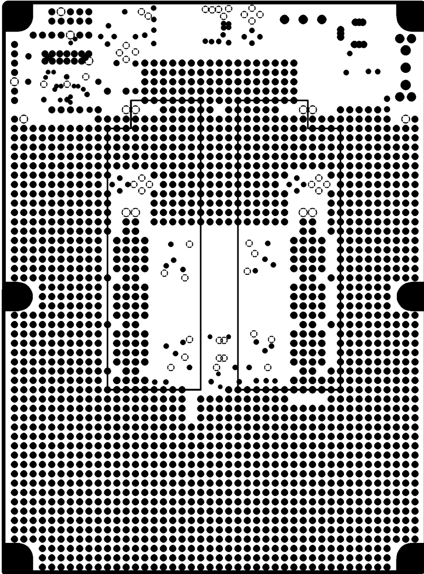
INTERNAL PLANE2
