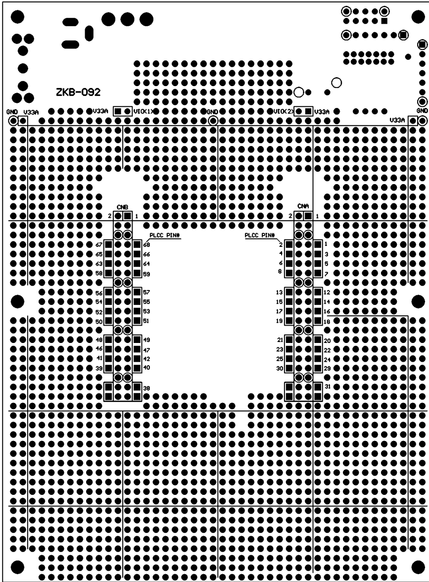
Solder Side
