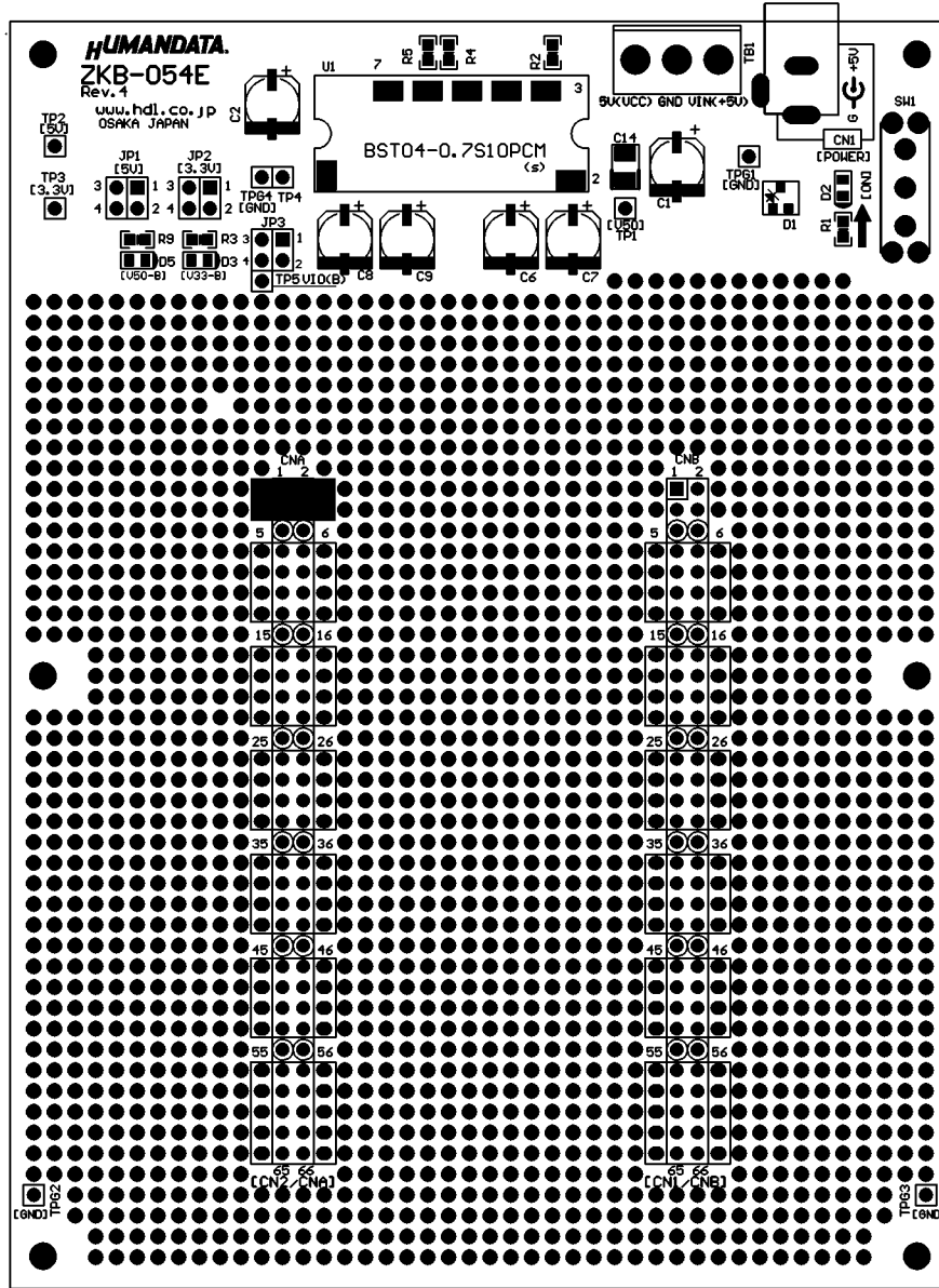
Component Side
