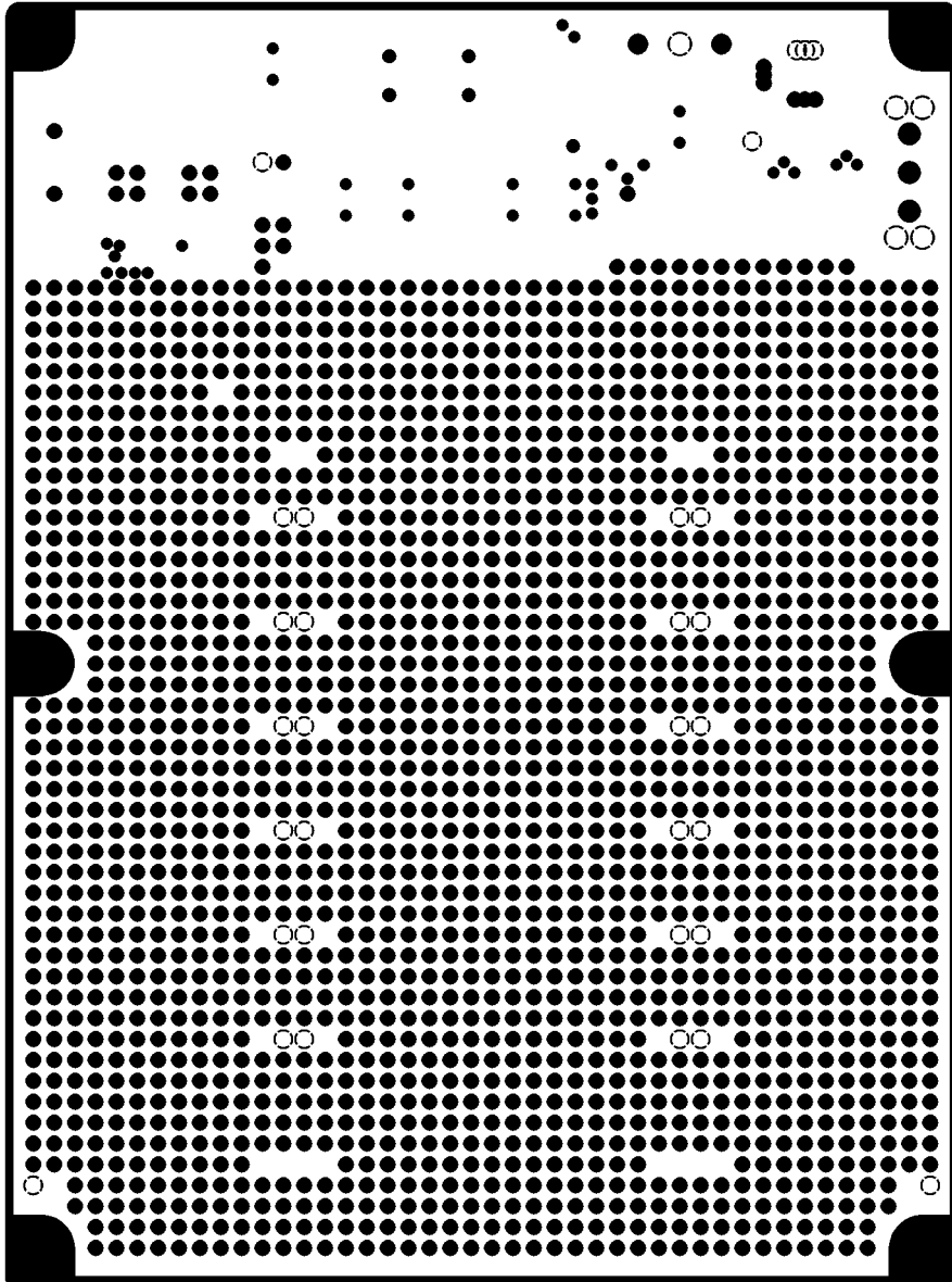
INTERNAL PLANE1
