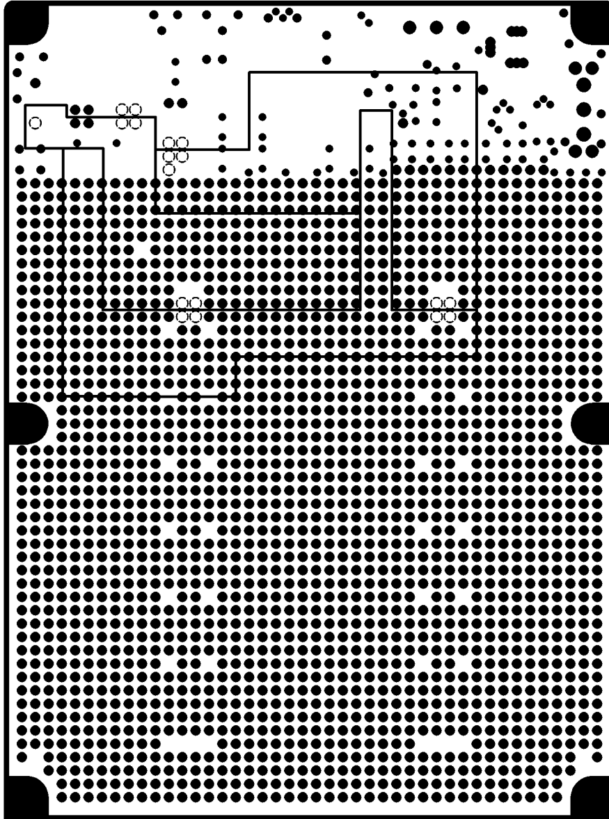
INTERNAL PLANE2
