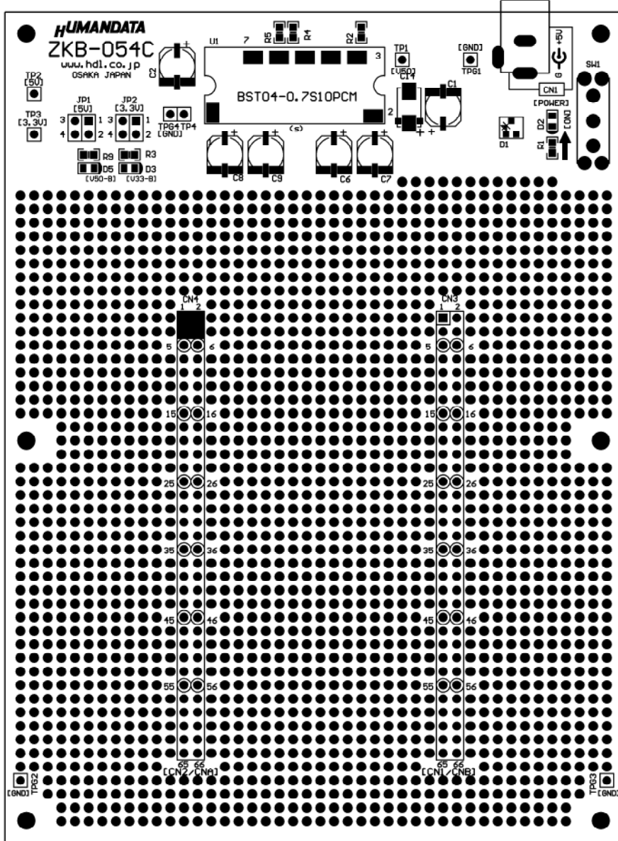
Component Side
