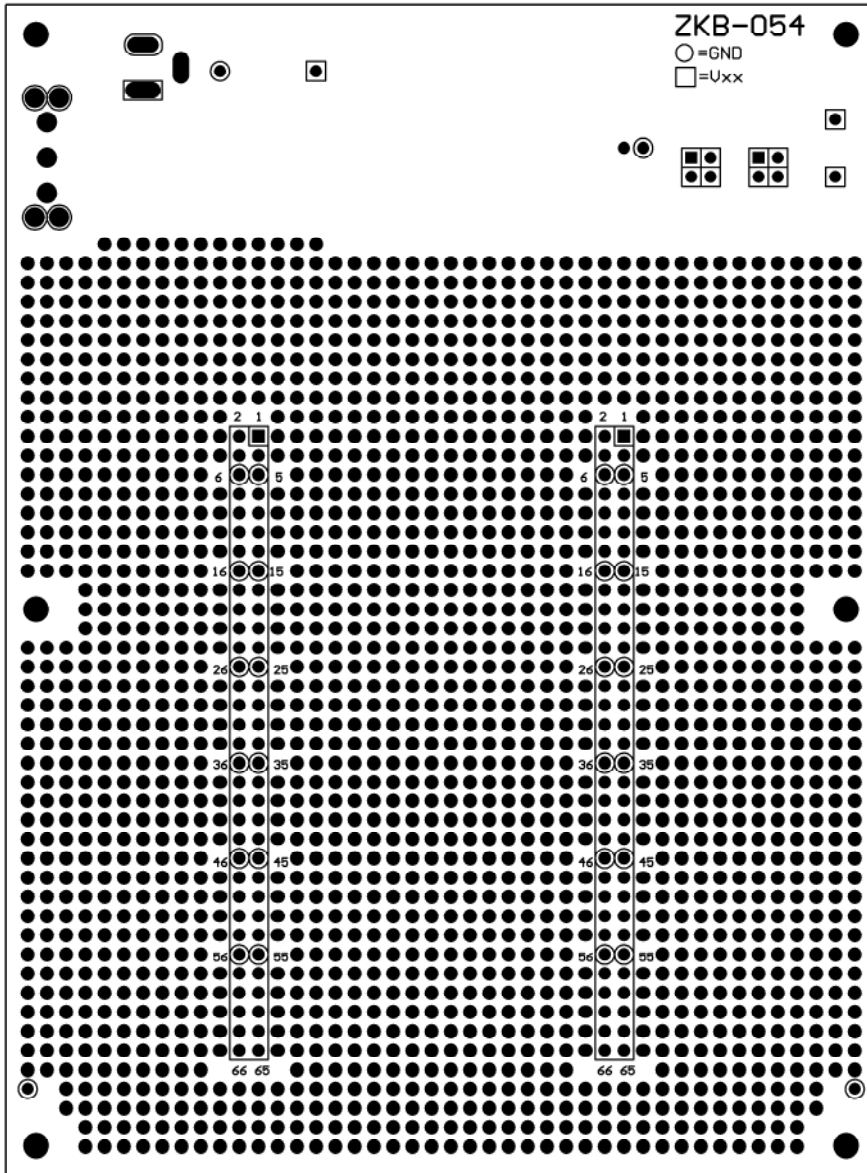
Solder Side
