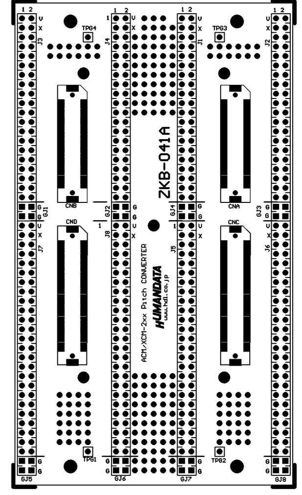
Component Side
