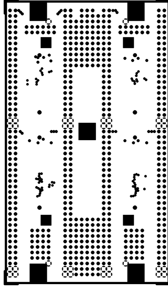
INTERNAL PLANE 2
