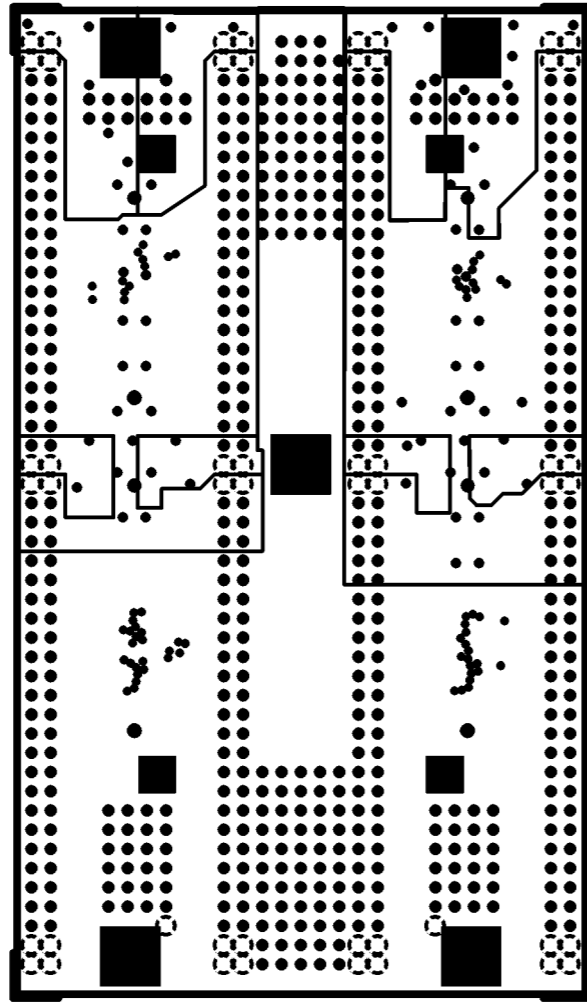
INTERNAL PLANE 1
