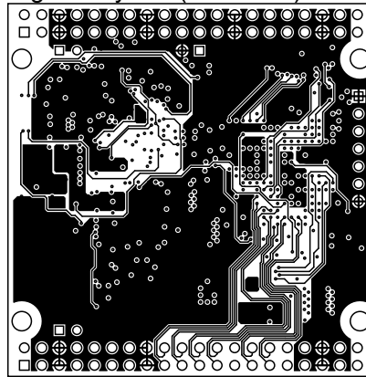
Signal Layer 1 (Scale 1:1)
