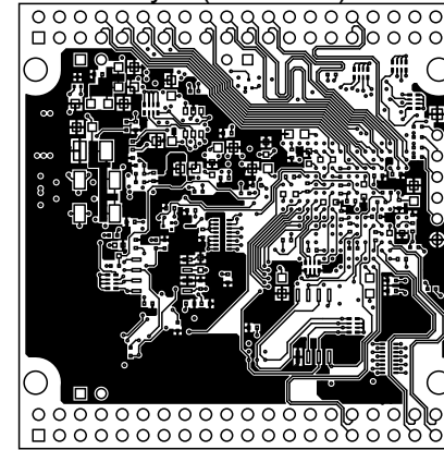
BottomLayer (Scale 1:1)
