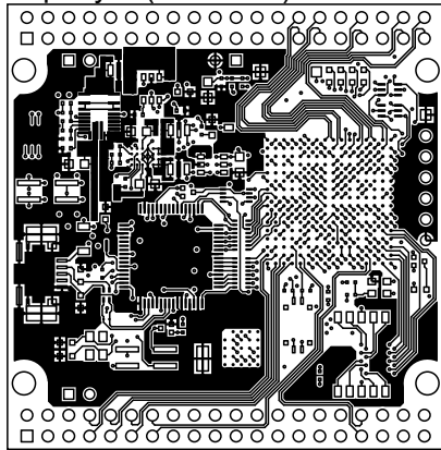
TopLayer (Scale 1:1)
