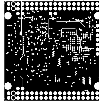
Internal Plane2 (Scale 1:1)
