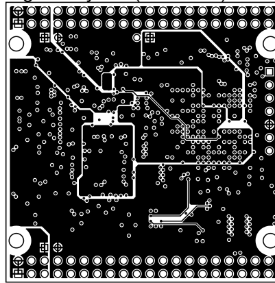
Signal Layer 2 (Scale 1:1)
