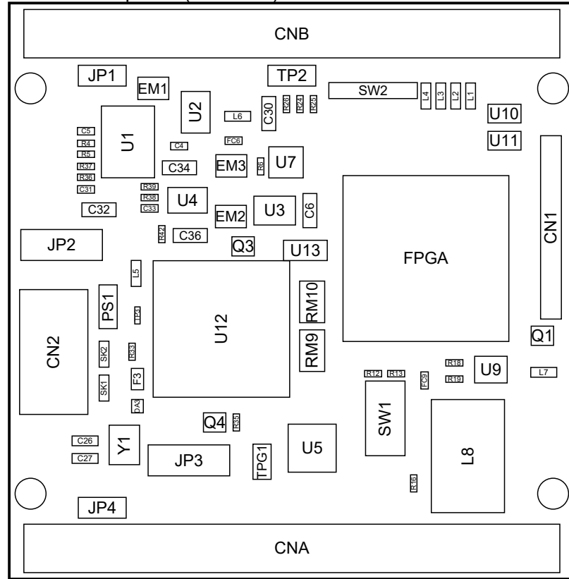
View from Top side (Scale 2:1)
