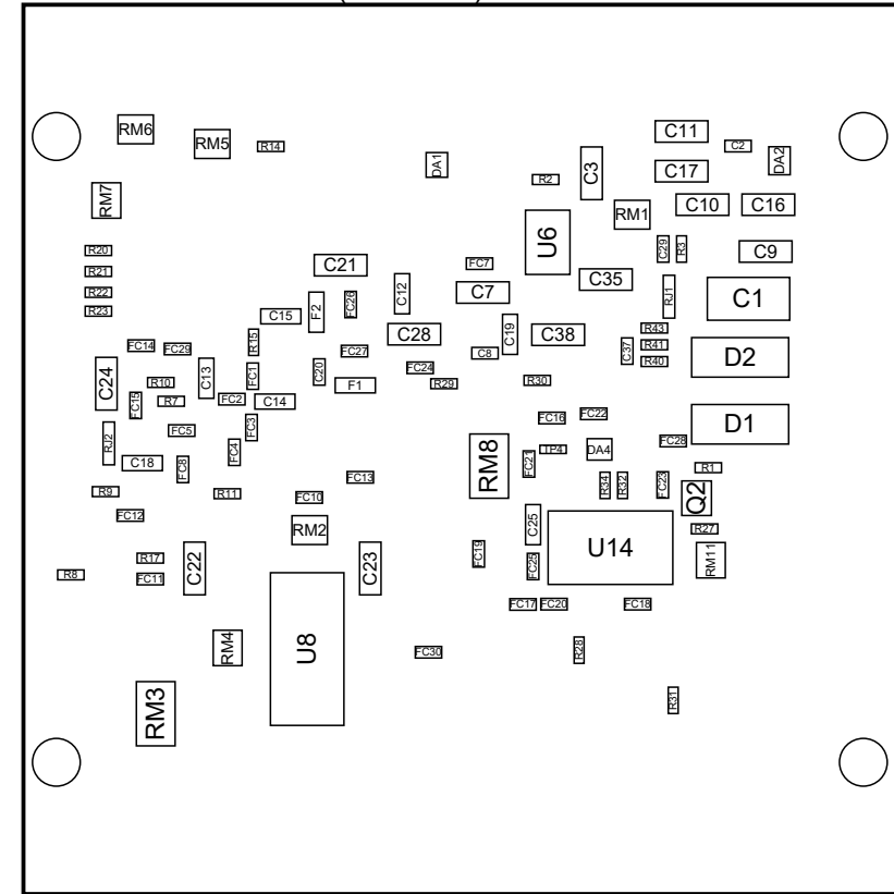
View from Bottom side (Scale 2:1)
