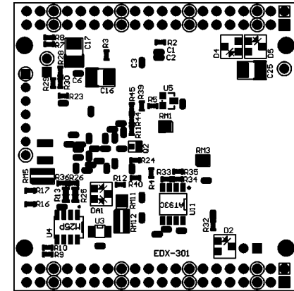
Solder Side
