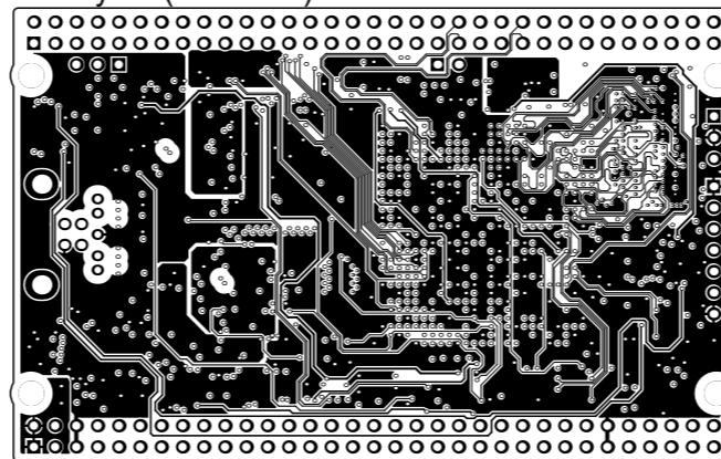
MidLayer2 (Scale 1:1)
