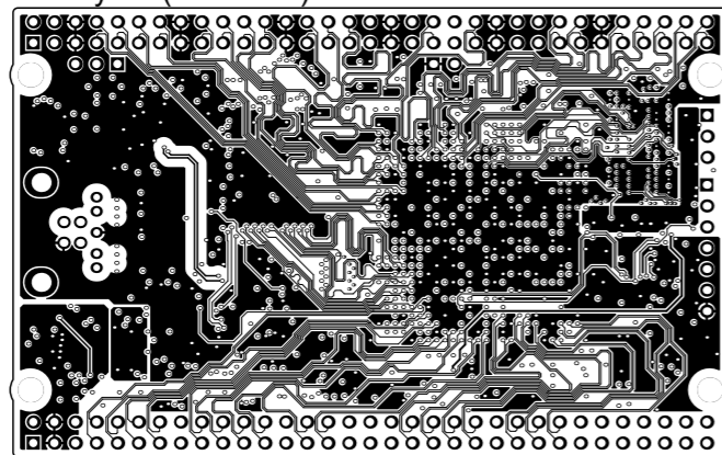
MidLayer1 (Scale 1:1)
