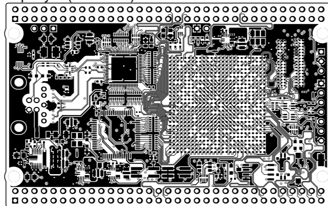
TopLayer (Scale 1:1)
