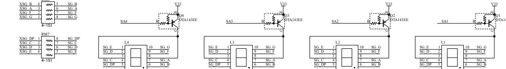
7 Segment LED
