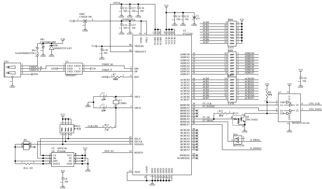
USB Controller
