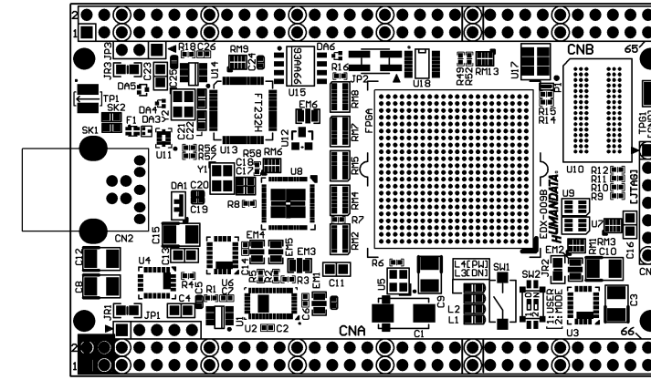
Component Side
