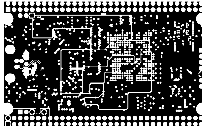
MID LAYER4
