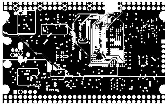
MID LAYER3
