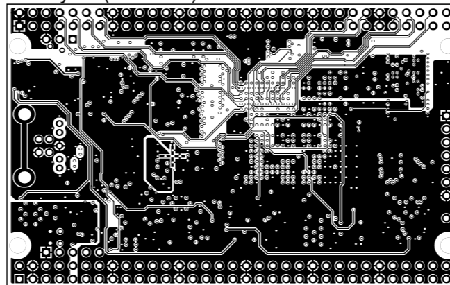
MidLayer3 (Scale 1:1)
