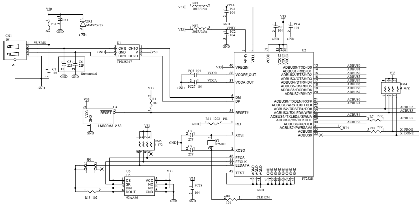
USB Controller
