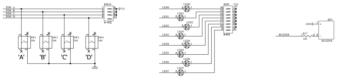
Push Switch
