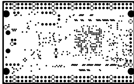
INTERNAL PLANE1
