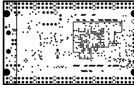
INTERNAL PLANE2
