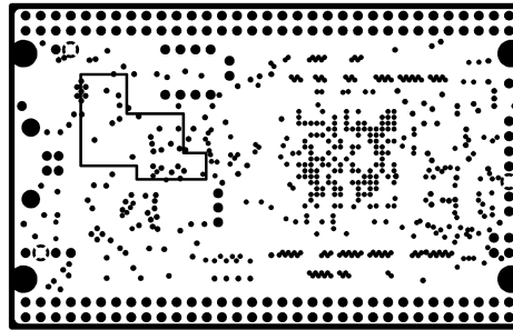
INTERNAL PLANE3
