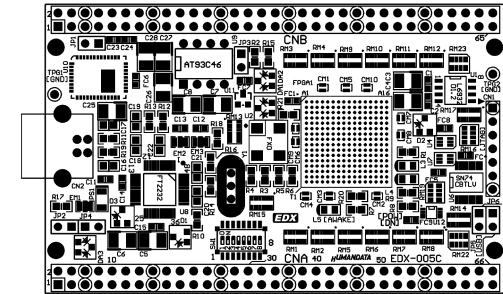
Component Side
