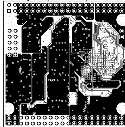
MidLayer2 (Scale 1:1)
