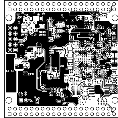
BottomLayer (Scale 1:1)
