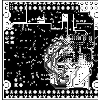
MidLayer2 (Scale 1:1)
