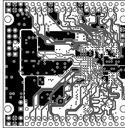
MidLayer1 (Scale 1:1)
