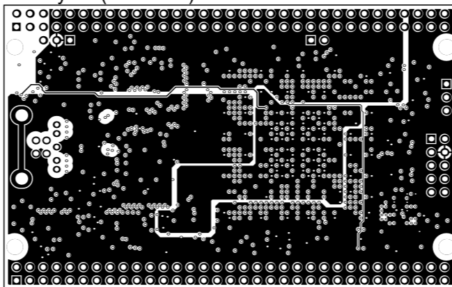
MidLayer2 (Scale 1:1)
