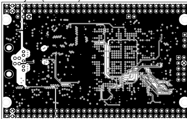
MidLayer1 (Scale 1:1)
