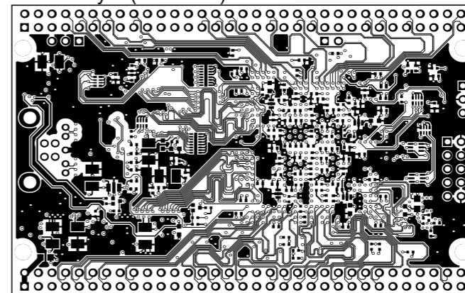
BottomLayer (Scale 1:1)
