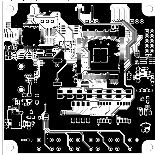
TopLayer (Scale 1:1)
