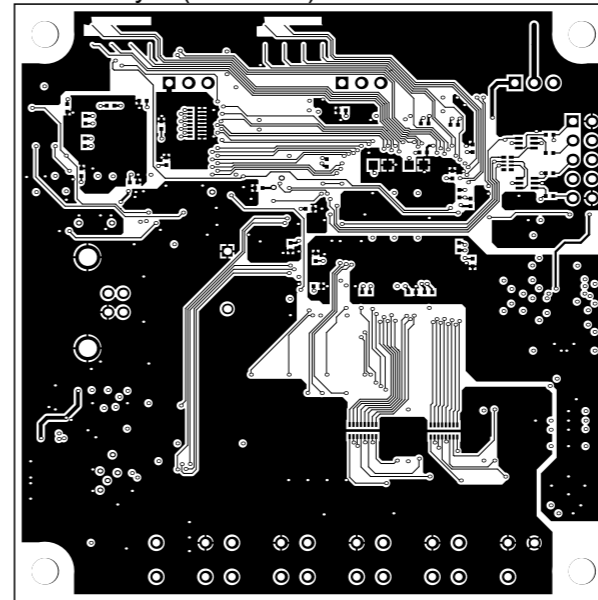
BottomLayer (Scale 1:1)
