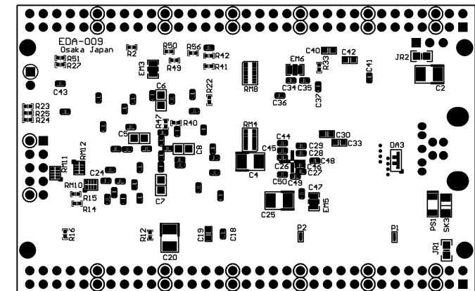
Solder Side
