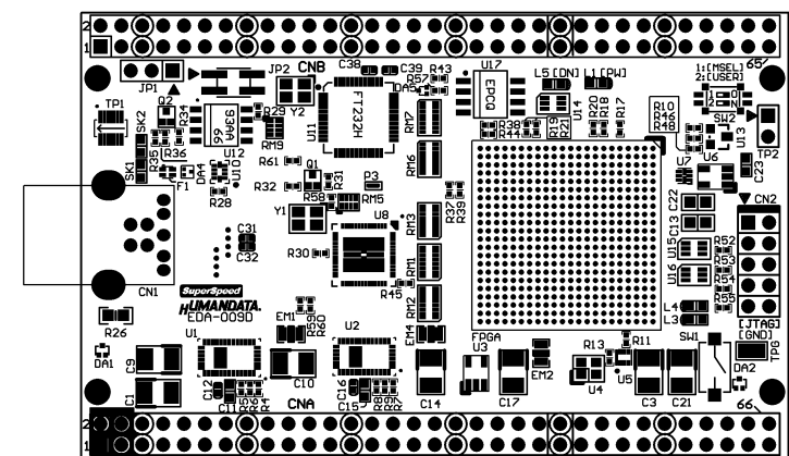
Component Side
