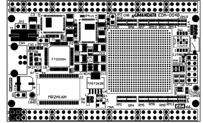
Component Side
