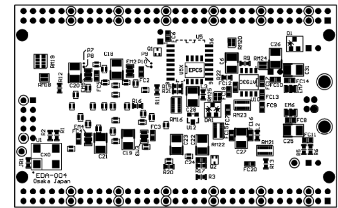
Solder Side
