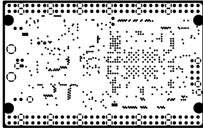
INTERNAL PLANE(GND)
