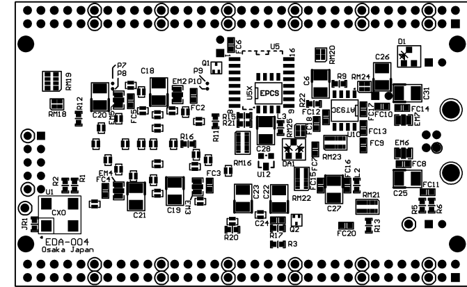
Solder Side
