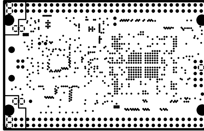
INTERNAL PLANE(VCC)
