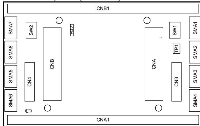
View from Top side (Scale 1:1)
