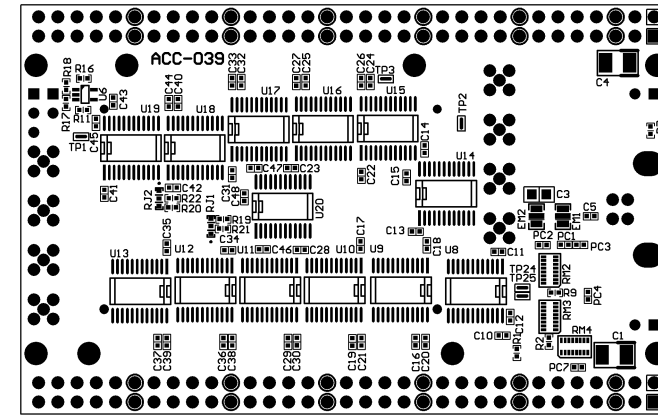
Solder Side
