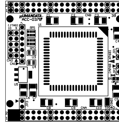
Component Side
