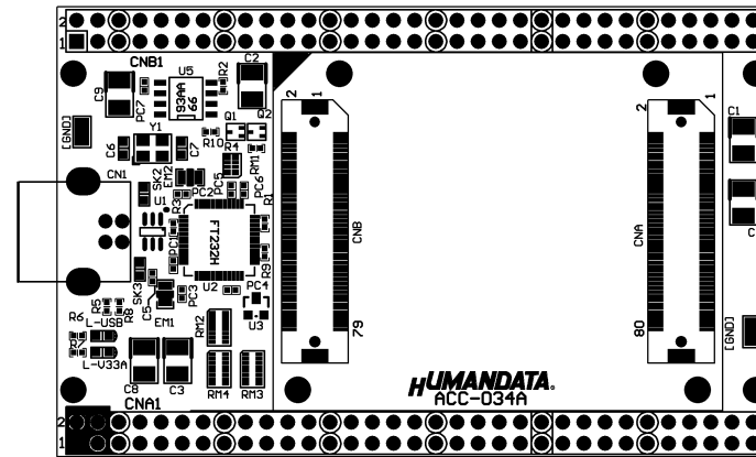
Component Side
