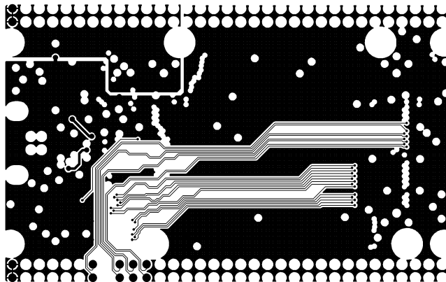
Signal Layer 1
