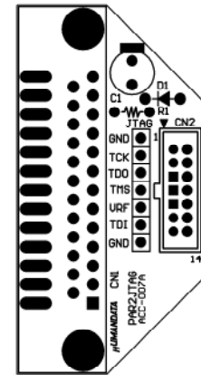
Component Side
