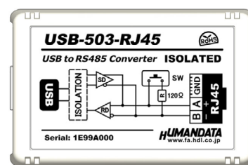
TOP side (Block diagram)
