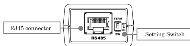
Rear Side (RS-485)
