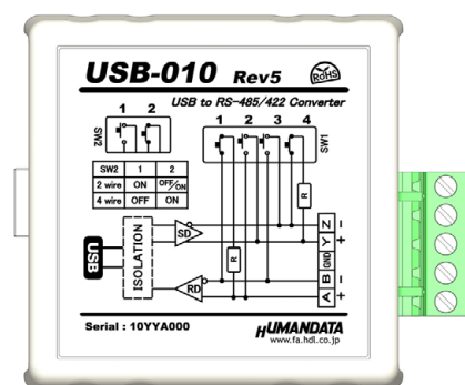
TOP side (Block diagram)
