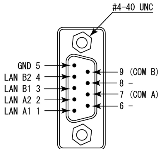
D-Sub 9pin Male
