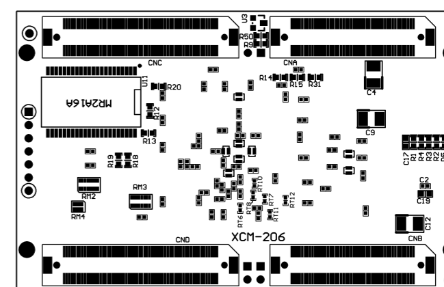
Solder Side
