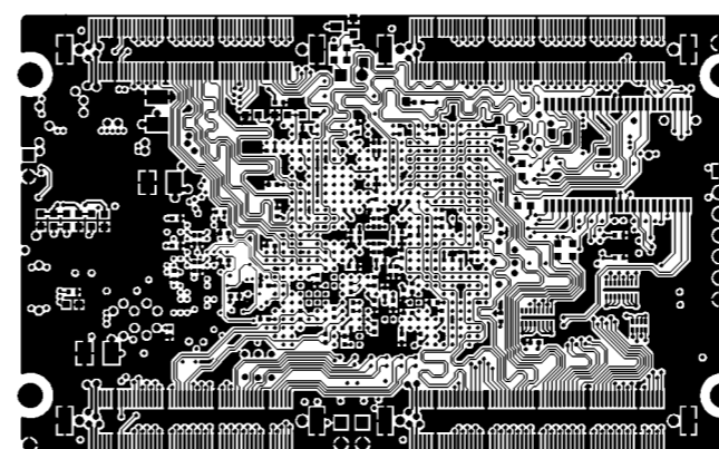
INTERNAL PLANE 2
