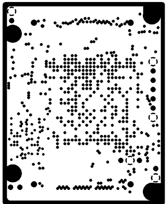
INTERNAL PLANE1
