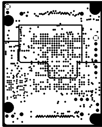
INTERNAL PLANE3
