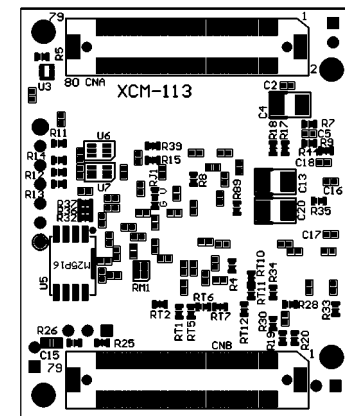
Solder Side
