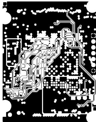
MID LAYER3
