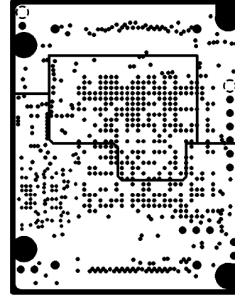
INTERNAL PLANE2
