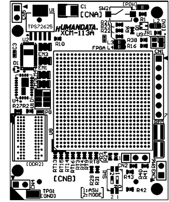
Component Side
