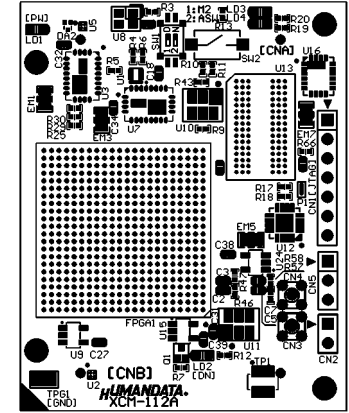
Component Side
