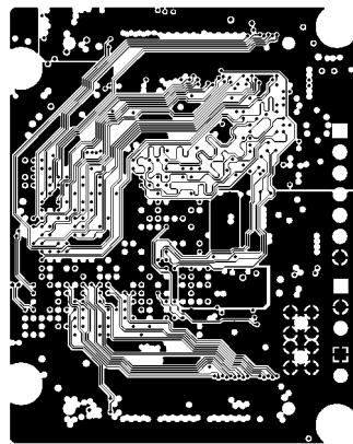
MID LAYER3
