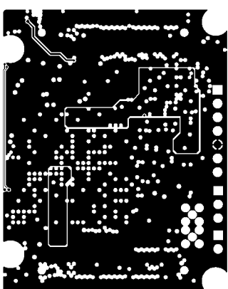
MID LAYER5
