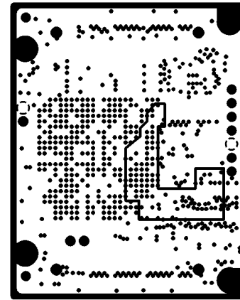
INTERNAL PLANE2
