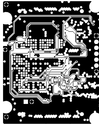
MID LAYER3
