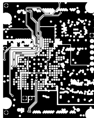
MID LAYER4
