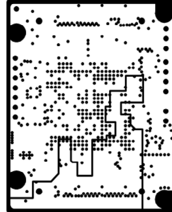
INTERNAL PLANE2(VCC)
